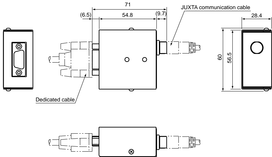
Figure 1.4.1 External View of the Communication Adapter
